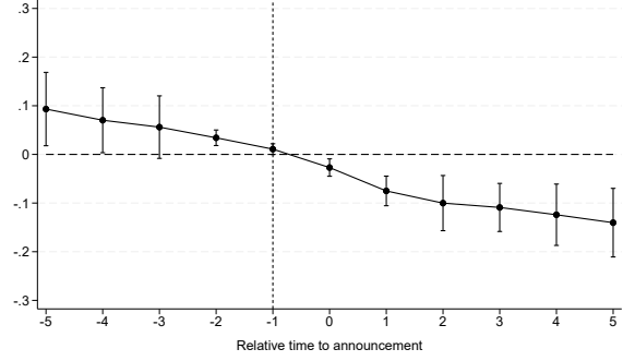
Panel B: Callaway and Sant'Anna universal base period
