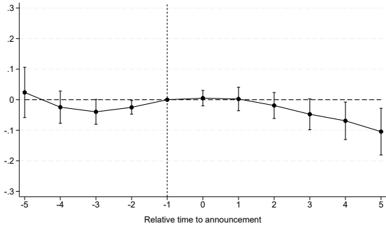
Panel C: TWFE
