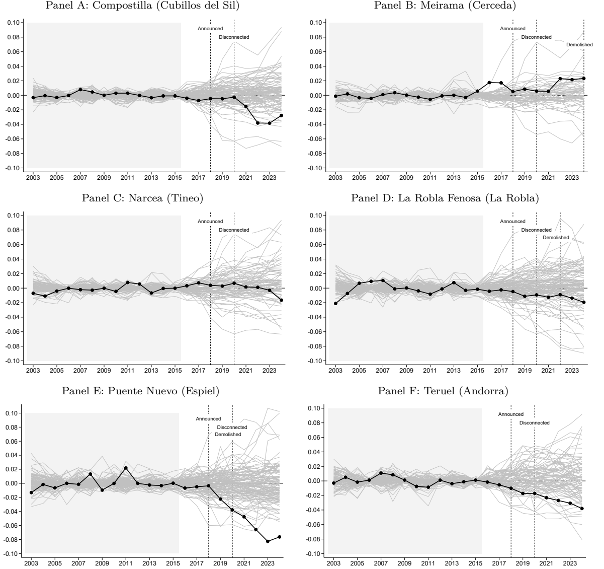
FIGURE D.17 PLACEBO-BASED INFERENCE: EMPLOYMENT
