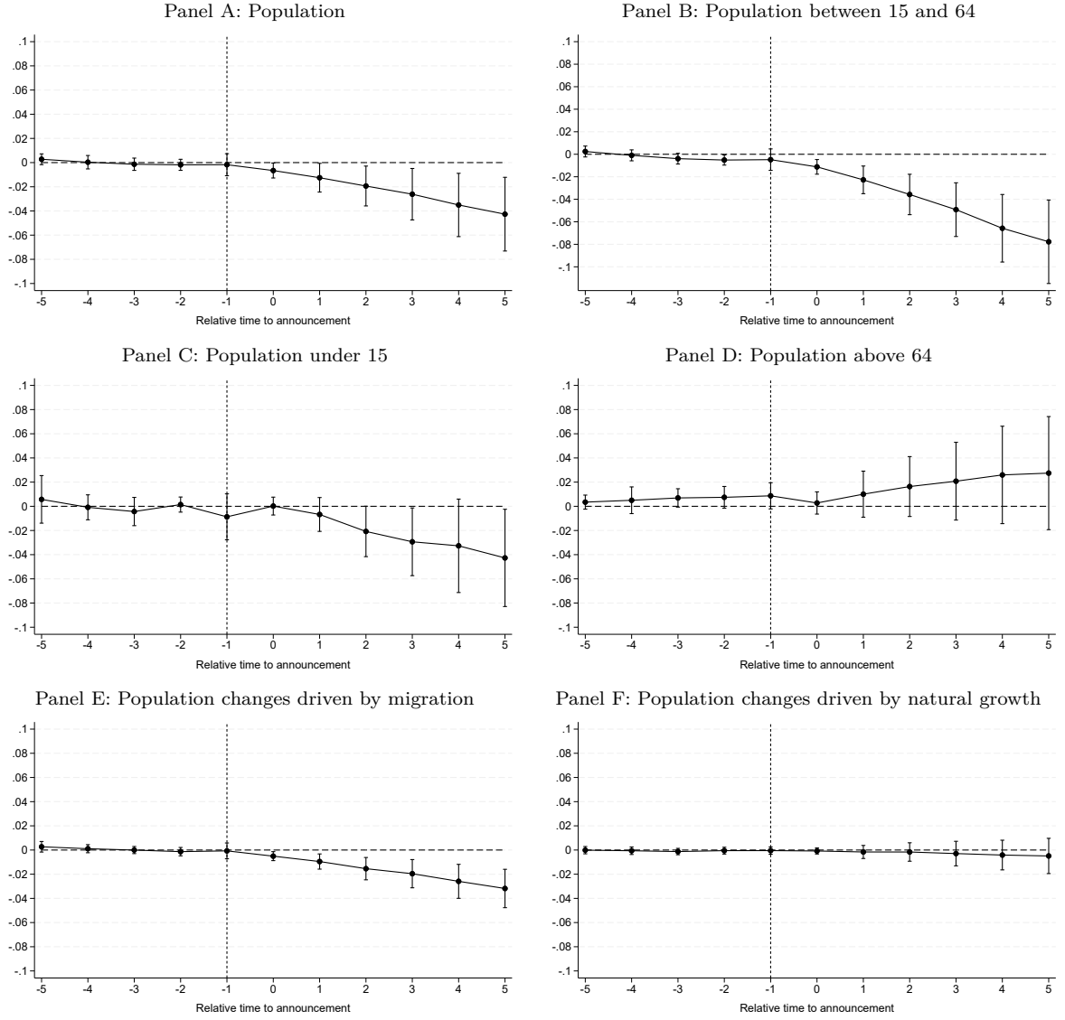
FIGURE 4 EVENT STUDY FOR POPULATION BY AGE AND DRIVER
