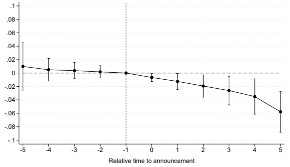
Panel D: Sun and Abraham
