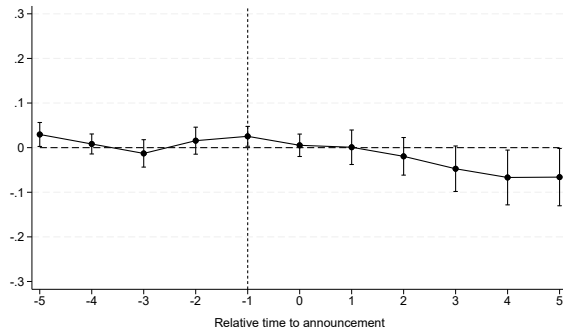
Panel A: Baseline (Callaway and Sant'Anna varying base period)
