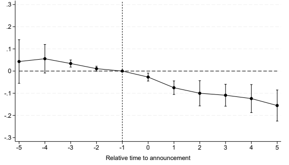
Panel D: Sun and Abraham
